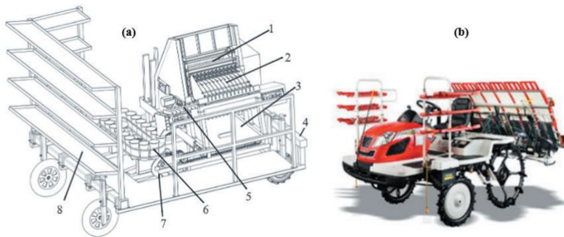
Figure 4: Automatic trans-planter.
