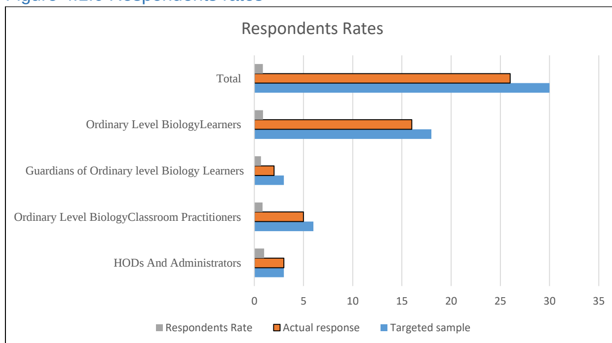
Figure 4.1.0 Respondents rates
